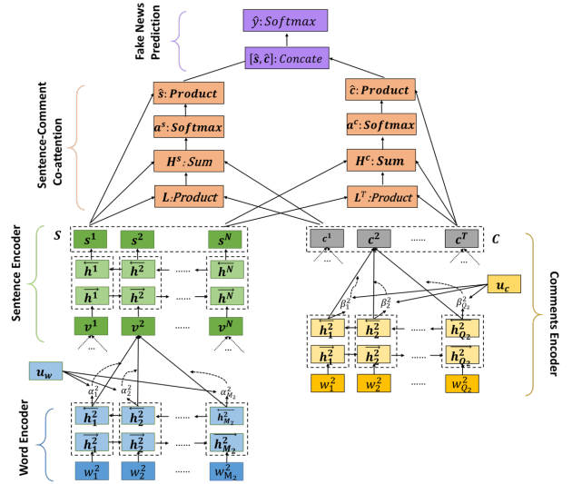
Figure 2: The proposed framework dEFEND consists of four components: (1) a news content (including word-level and sentence-level) encoder, (2) a user comment encoder, (3) a sentence-comment co-attention component, and (4) a fake news prediction component.
