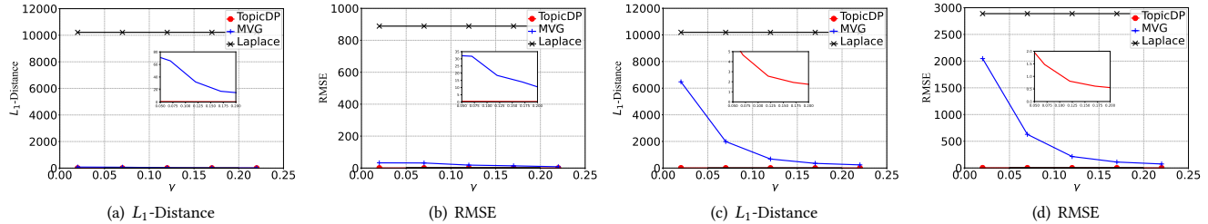
Figure 4: L_1 -Distance and RMSE vs \gamma on the Enron Email Dataset (a, b) and Amazon Product Review Dataset (c, d).
