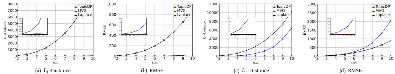
Figure 5: L_1 -Distance and RMSE vs Matrix Size with Fixed \epsilon = 3 on the Enron Dataset (a, b) and Amazon Dataset (c, d).
