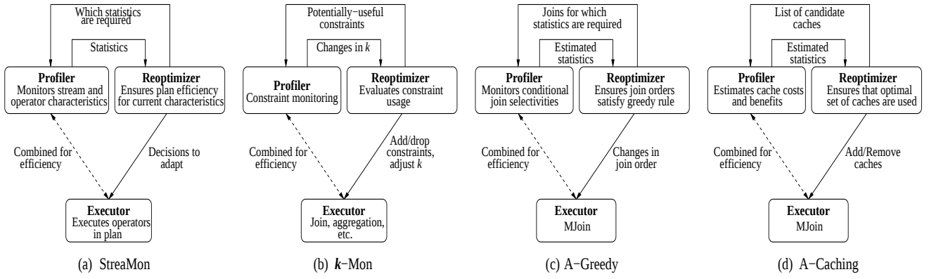
Figure 2: Basic structure of StreaMon, k -Mon, A-Greedy, and A-Caching
