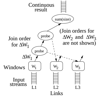
Figure 1: Plan for example query
