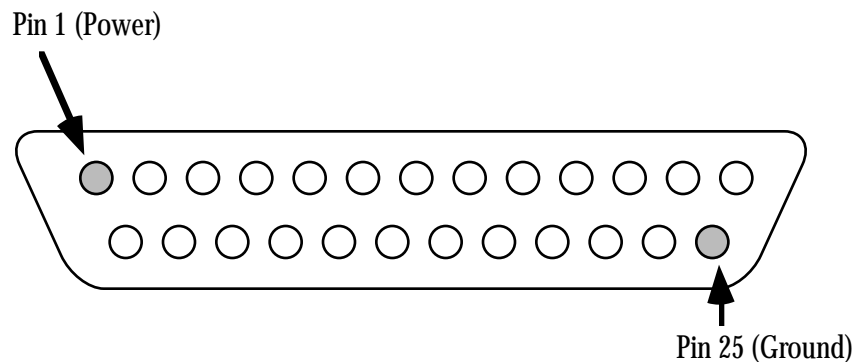
Power and Ground Lines on the DB25F connector (Back View)
