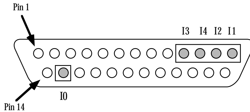
Data Input Lines on the DB25F connector (Back View)
