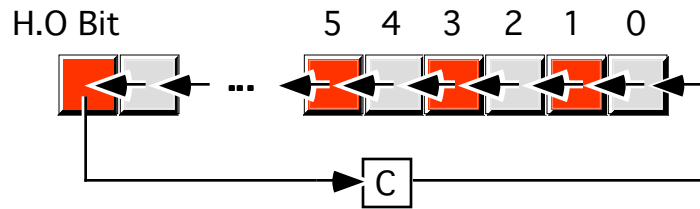
Rotate Through Carry Left Operation
