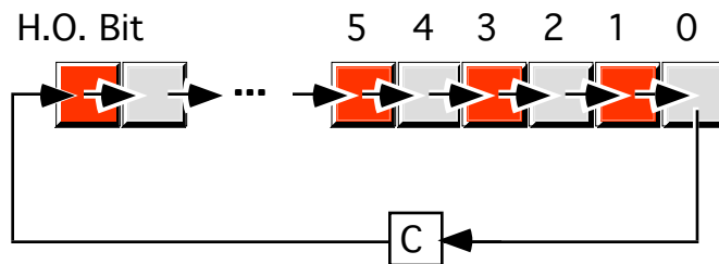
Rotate Through Carry Right Operation
