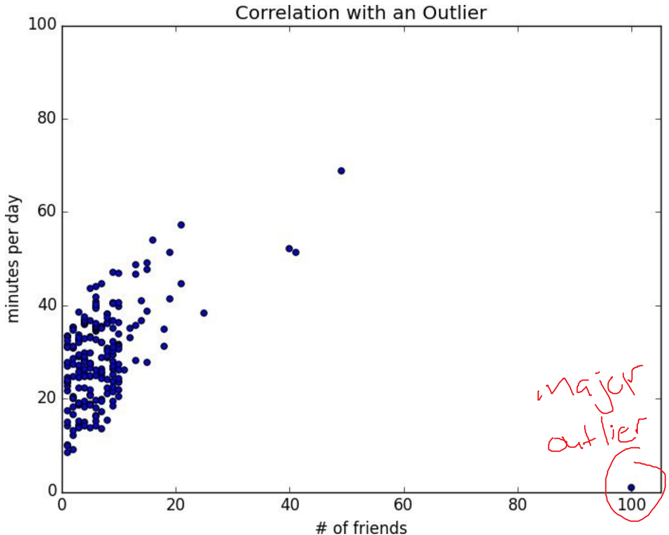
Figure 5-2. Correlation with an outlier
